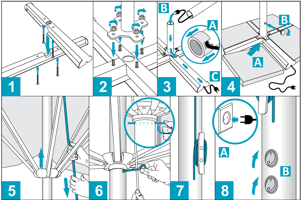
Fig. 2. Mounting process
